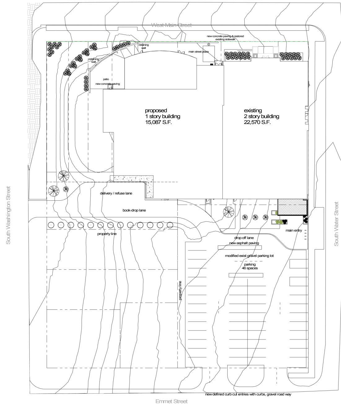
⊕ 2 SD site plan 1" = 20'-0"
